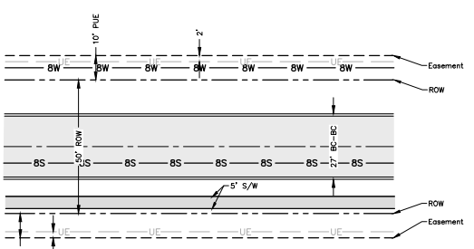
Typical Utility Layout
